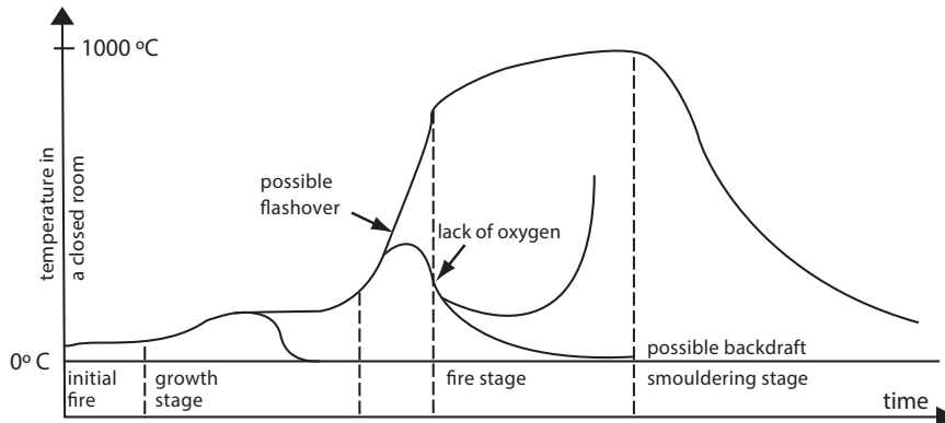
Figure 70 Fire curve
